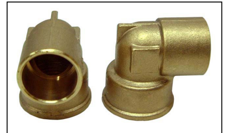
Product Code BRCFD2022B Unit EACH Description ELBOW FXC 22MMX3/4" SOLDER TYPE
