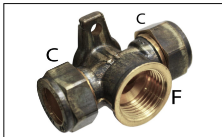
Product Code BRCF2024C Unit EACH Description BRASS TEE WALL PLATE 15MM C X C X F (SABS)
