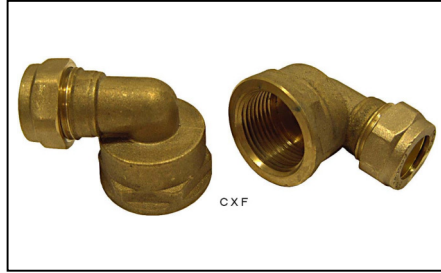
Product Code BRCF2022R Unit EACH Description REDUCE ELBOW 2022R 15MM X 22MM C X F ( COUPLER X FEMALE )
