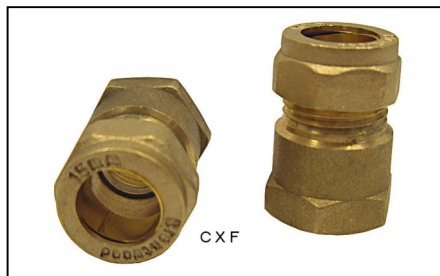
Product Code BRCF2002A Unit EACH Description COUPLER FEMALE IRON 2002A 15mm ( C X F ) COUPLER X FEMALE BRENTWOOD
