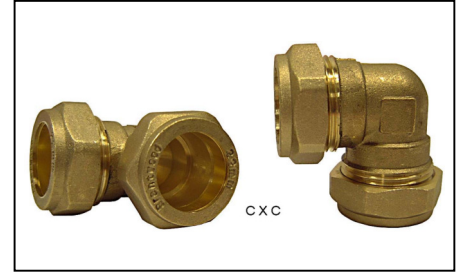
Product Code BRCF2020B Unit EACH Description ELBOW COPPER 2020B 22mm C X C (COPPER X COPPER ) BRENTWOOD
