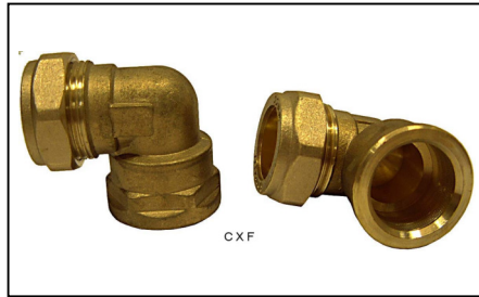
Product Code BRCF2022B Unit EACH Description ELBOW FEMALE 22MM 2022B F X C ( FEMALE X COUPLER )
