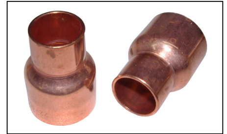
Product Code BRCFD102R Unit PACK Description COUPLER REDUCER 10'S 22X15, C X C, SOLDER TYPE
