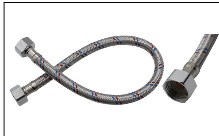
Product Code BRTAP02A Unit EACH Description BASIN HOSE 15MM X 15MM X 450MM
