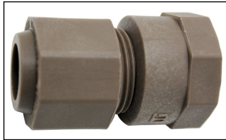
Product Code BRUNI2002R Unit EACH Description PLASTIC FEMALE COUPLER REDUCE 15MM X 22MM (UNITWIST)
