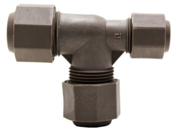
Product Code BRUNI2044R Unit EACH Description PLASTIC TEE REDUCE 22MM X 15MM X 22MM (UNITWIST)
