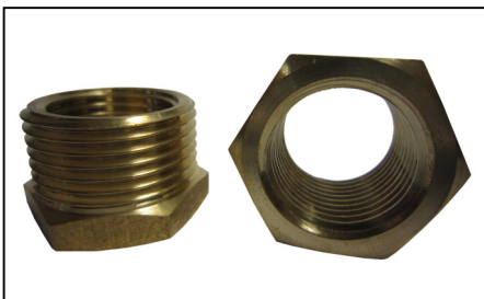
Product Code BRCF2003R Unit EACH Description REDUCER BUSH 15X22mm F X M CHROM
