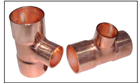
Product Code BRCFD3912R Unit PACK Description T REDUCER 22X15X22mm SOLD 10'S SOLDER TYPE
